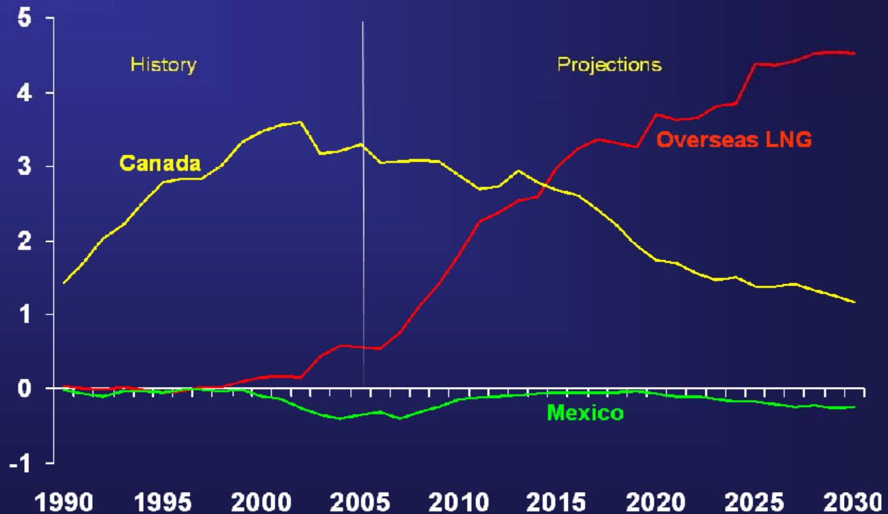
U.S. Net Imports of Natural Gas, 1990-2030 (trillion cubic feet)
