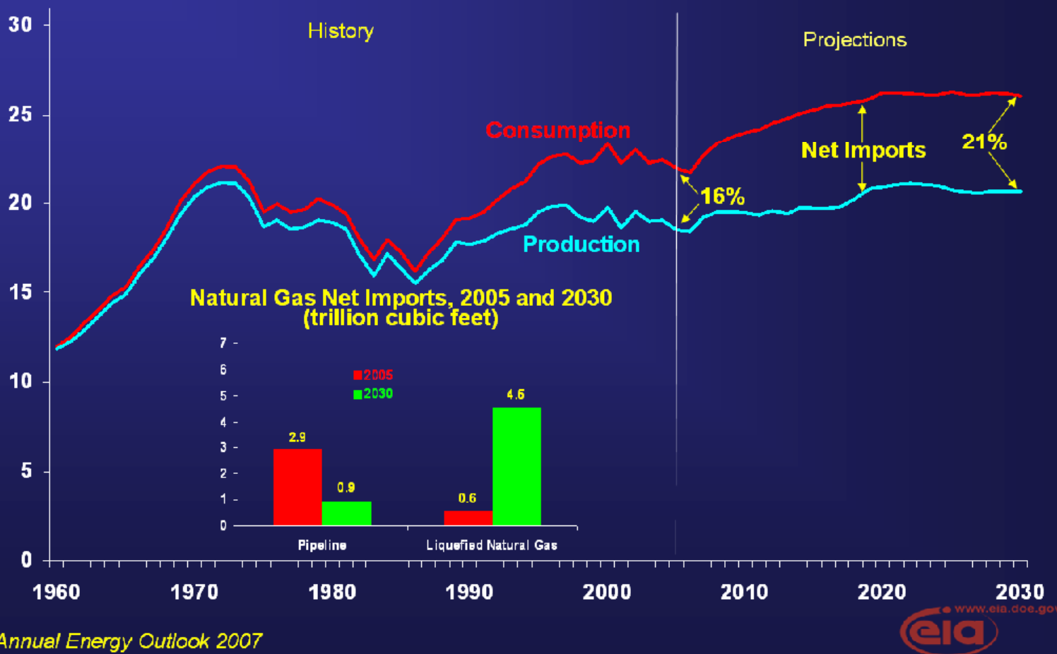
U.S. Natural Gas Production, Consumption, and Net Imports, 1960-2030 (trillion cubic feet)
